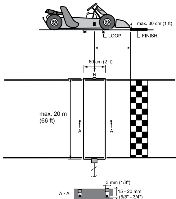
Figure 2.1 Detection loop installation overview
