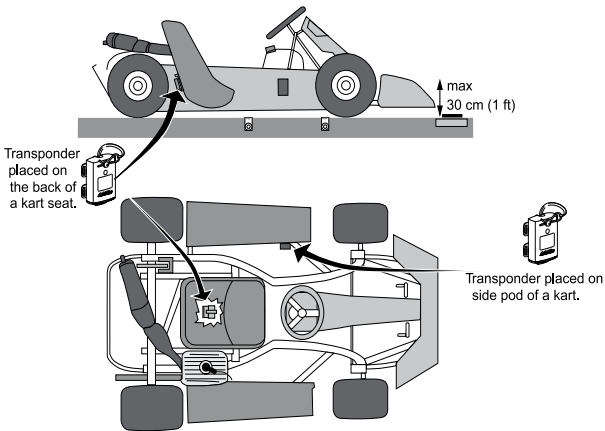
Figure 3.1 Transponder placement
